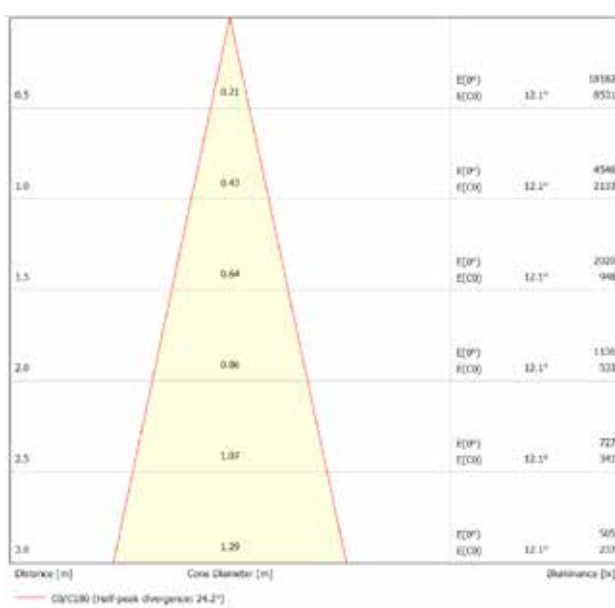
Diagramma a cono Cone diagram
